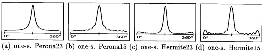
Fig. 8. Depicted is the energy of the responses of the one-sided Hermite function and one-sided Perona's function for an horizontal endstopping. To demonstrate the effect of approximations with only a few basis functions the responses for 15 and for 23 basis functions are shown. The main effect of taking less basis functions is not a worse orientation selectivity but strong ripples. The same is true for the two-sided original functions.
