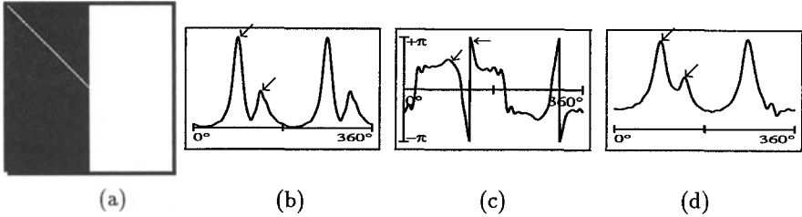
Fig. 2. (a) junction, (b) energy, (c) phase for the double Hermite function. (d) energy for the one-sided function. The energy shows two events at 90^\circ and 136^\circ (modulo 180^\circ ). The phase at the orientation of the maxima of the energy (1.77 and 3.00) reveals that they originate from a line at 136^\circ and an edge at 90^\circ . Due to the influence of the dominating edge the maximum of the line is shifted by less than one degree. The missing second peak of the line at 316^\circ in (d) shows that it terminates at the keypoint. The center of the double Hermite function matches the keypoint within 1 pixel.
