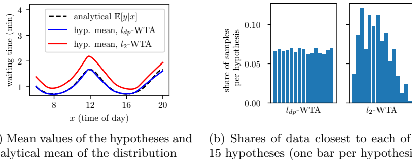
Fig. 3: Further statistics computed on the models for the call center example.
