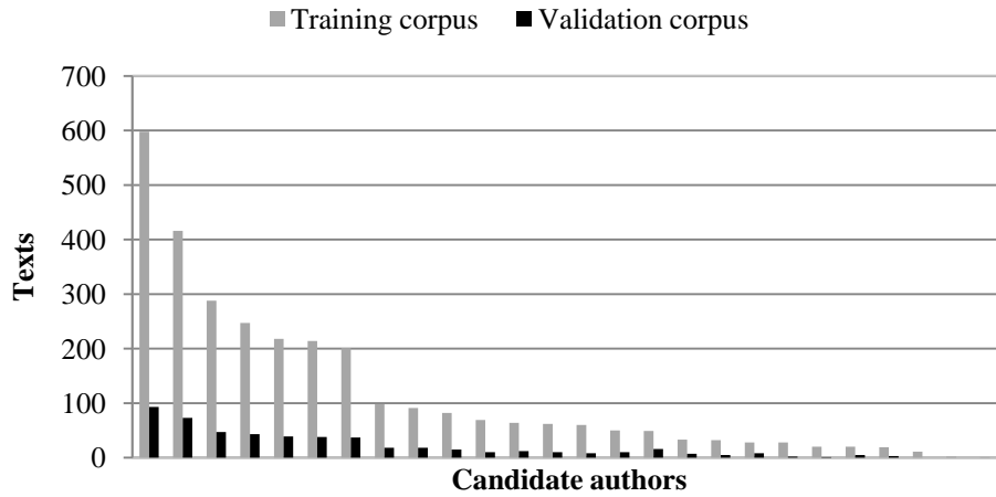
Fig. 4. Distribution of the training/validation corpus of the PAN11-AA-Small.
