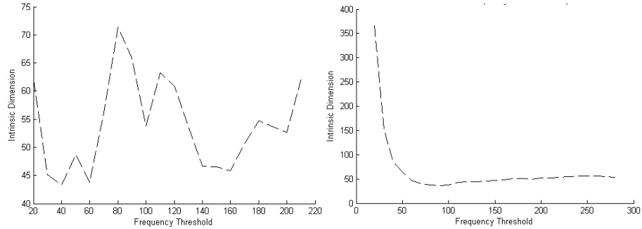
Fig. 6. Intrinsic dimension of PAN11-AA-Small (left) and PAN11-AA-Large (right) for varying freq. threshold.
