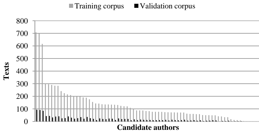
Fig. 5. Distribution of the training/validation corpus of the PAN11-AA-Large.
