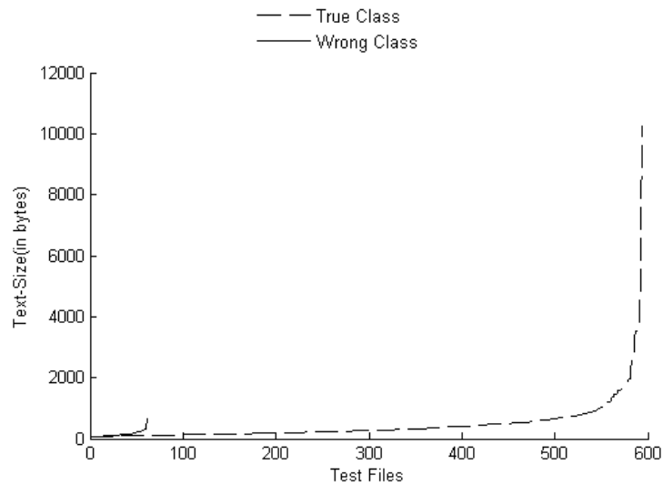
Fig. 7. Text-size distribution of PAN-11-AA-Large validation corpus where CNG and SVM predictions agree.
