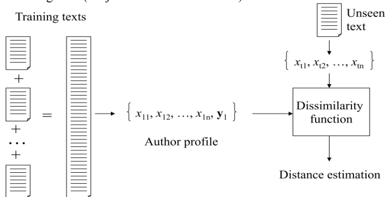
Fig. 1. Overview of the CNG method (only one candidate author is shown).
