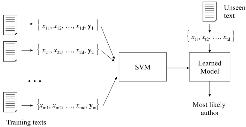
Fig. 2. Overview of the SVM method.
