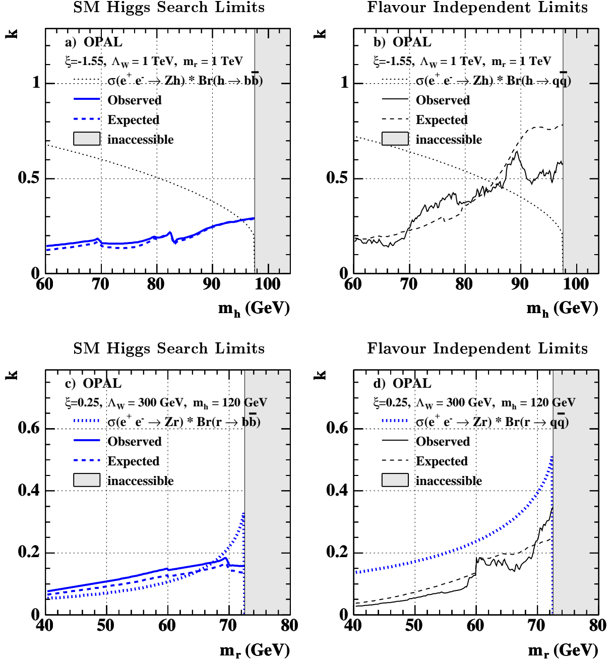
Figure 4: The cross-section times branching ratio of the Higgs-like (Figure a and b) and radion-like state (Figure c and d) relative to the cross-section of SM Higgsstrahlung together with the observed and expected limits (solid and dashed lines) obtained from the SM (Figure a and c) and the flavour independent (Figure b and d) Higgs boson searches at one point in the Randall-Sundrum parameter space as a function of the mass of the Higgs-like state m_h and the mass of the radion-like state m_r . The dotted lines in Figures a and c indicate the cross-section times \text{Br}(r \text{ or } h \rightarrow b\bar{b}) and in Figures b and d the cross-section times \text{Br}(r \text{ or } h \rightarrow \text{hadrons}) . The shaded region is inaccessible by the theory. Model points are excluded if the predicted cross-section times branching ratio exceeds the limit.
