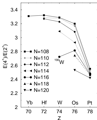
FIG. 4. Systematics of the ratio of the first 4^+ and 2^+ level energies in heavy, rare earth nuclei.
