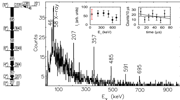
FIG. 2. Proposed decay scheme and delayed \gamma -ray spectra for ^{190}\text{W} with the condition that the \gamma -rays were detected between 1 and 70 \mu\text{s} after the ion implantation. The insets show the relative intensities and the summed time spectrum associated with the labelled transitions. The two lines on the time spectrum correspond to the upper and lower limits for the lifetime of \tau=4.5 ms and \tau=135 \mu\text{s} , respectively.
