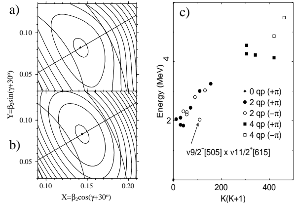
FIG. 3. Potential energy surface calculations for (a) the ground-state configuration and (b) the K^\pi = 10^- configuration for ^{190}\text{W} . The energy difference between two successive contour lines is 200 keV. (c) Blocked BCS calculations for ^{190}\text{W} , showing the favoured nature of the K^\pi = 10^- two quasineutron configuration.
