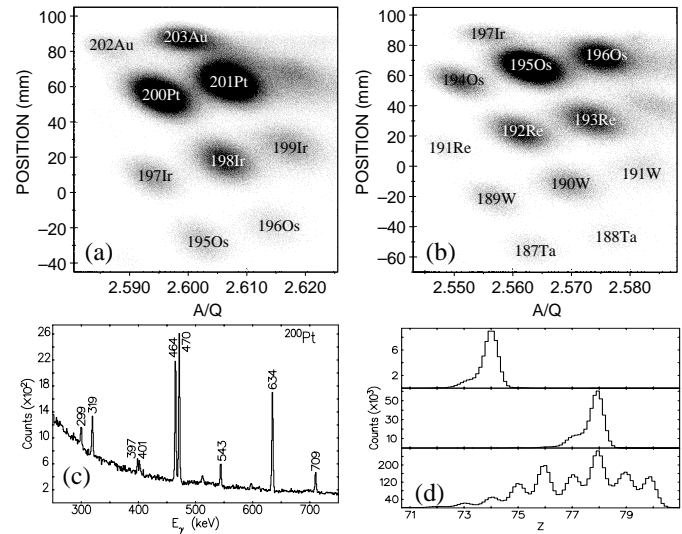
FIG. 1. Identification plot of the fragments by the FRS for (a) hydrogen like ions ( Q=Z-1 ) and (b) fully stripped ions ( Q=Z ) for the setting centred on fully stripped ^{191}\text{W} . Panel (c) shows the gamma-spectrum recorded in coincidence with the events labeled as ^{200}\text{Pt} in (a). All the \gamma -rays belong to ^{200}\text{Pt} . The strongest transitions were already known [17]; the others were found in the present experiment and proved to belong to ^{200}\text{Pt} by \gamma - \gamma coincidence measurement. (d) Z spectra obtained from the ionization chamber. From below: total Z spectrum, events corresponding to the ^{200}\text{Pt} in (a) and events corresponding to ^{190}\text{W} in (b). As the latter two spectra show, there is a small contamination from nuclei with Z-1 , namely ^{A-5}X_{Z-1} [10], which can be removed by gating on the ionisation chamber.
