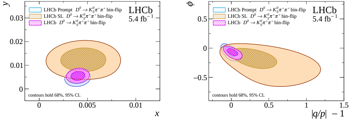
Figure 5: Two-dimensional 68% and 95% confidence-level contours on (left) (x, y) and (right) (|q/p| - 1, \phi) . Results from Run 2 D^{*+} \rightarrow D^0(\rightarrow K_S^0 \pi^+ \pi^-) \pi^+ (Prompt) [9], \bar{B} \rightarrow D^0(\rightarrow K_S^0 \pi^+ \pi^-) \mu^- \bar{\nu}_\mu X (SL), and their combination are shown.
