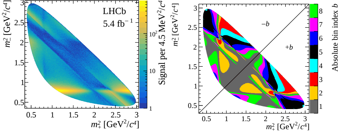
Figure 1: (Left) D^0 Dalitz plot of reconstructed \bar{B} \rightarrow D^0(\rightarrow K_S^0 \pi^+ \pi^-) \mu^- \bar{\nu}_\mu X decays for the D^0 flavor and (right) definition of the binning scheme proposed by CLEO [23].
