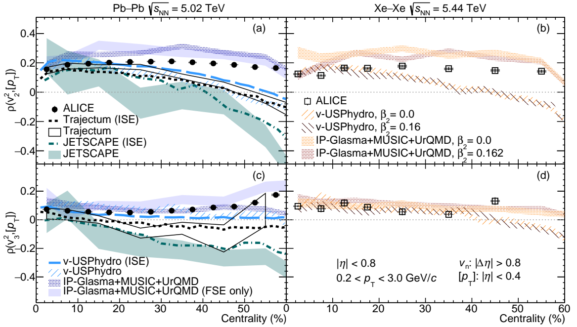
Figure 1: Centrality dependence of \rho(v_2^2, [p_T]) (top) and \rho(v_3^2, [p_T]) (bottom) in Pb–Pb collisions at \sqrt{s_{NN}} = 5.02 TeV (a,c) and Xe–Xe collisions at \sqrt{s_{NN}} = 5.44 TeV (b, d). The statistical (systematic) uncertainties are shown as vertical bars (filled boxes). The initial-state estimations (ISE) are represented by lines, while IP-Glasma+MUSIC+UrQMD [31], v-USPhydro [45], Trajectum [35], and JETSCAPE [36] hydrodynamic model calculations are shown with hatched bands.
