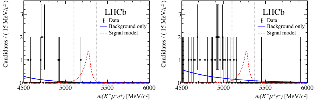
Figure 2: Invariant-mass distributions of the (left) B^+ \rightarrow K^+ \mu^- e^+ and (right) B^+ \rightarrow K^+ \mu^+ e^- candidates obtained on the combined data sets recorded in 2011 and 2012 with background only fit functions (blue continuous line) and the signal model normalised to 10 candidates (red dashed line) superimposed. The signal window is indicated with grey dotted lines. Difference between the two distributions arises from the effect of the m(K^+ \ell^-) requirement.
