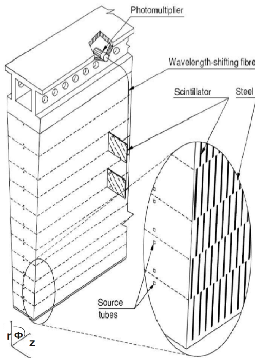
Figure 3.7: The TileCal module [38].
