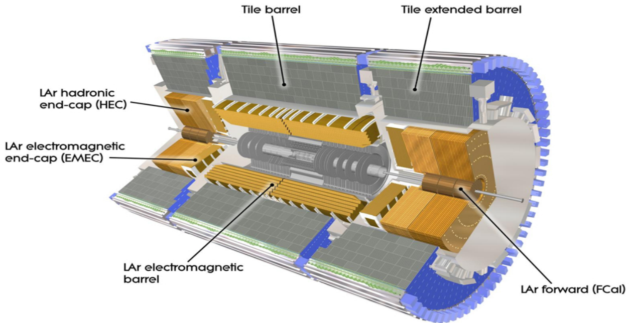
Figure 3.6: A part of the ATLAS detector, showing the hadronic calorimeters and the EM calorimeters [1].
