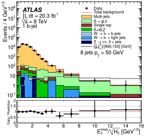
(c) 8j50, exactly one b -jet
