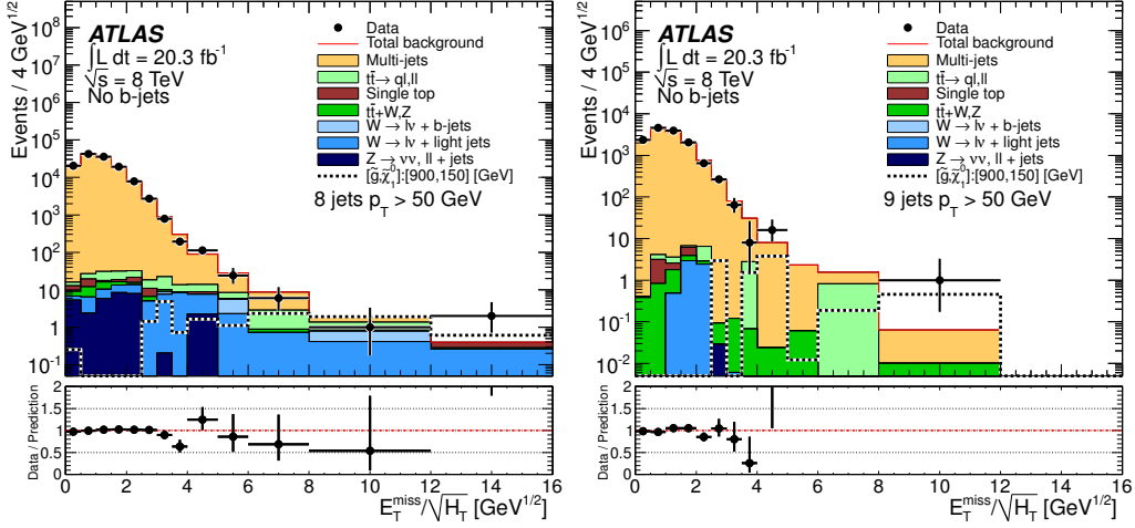
(a) 8j50, no b -jets
