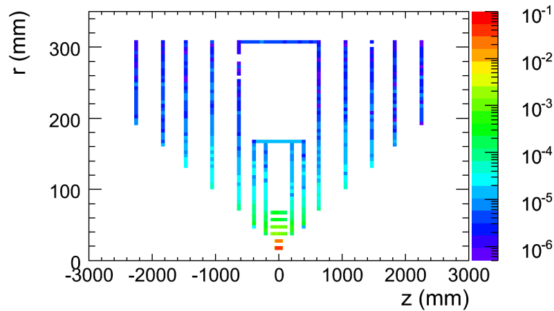
FIGURE 6.7-10. Distribution of the background hit densities on the inner silicon detectors (VTX, SIT, FTD) in units of [hits/mm 2 /BX].
