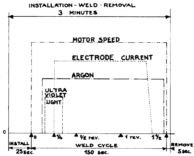
Fig. 8. Graph of weld cycle.
