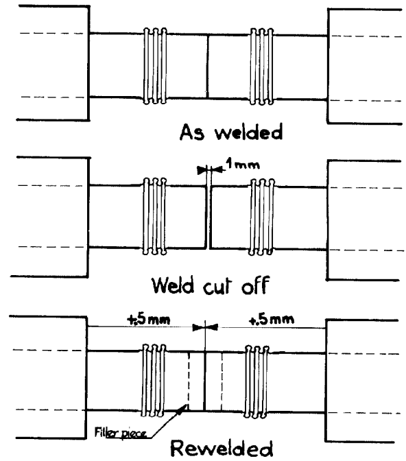
Fig. 7. Schematic of butt-weld tube joint.
