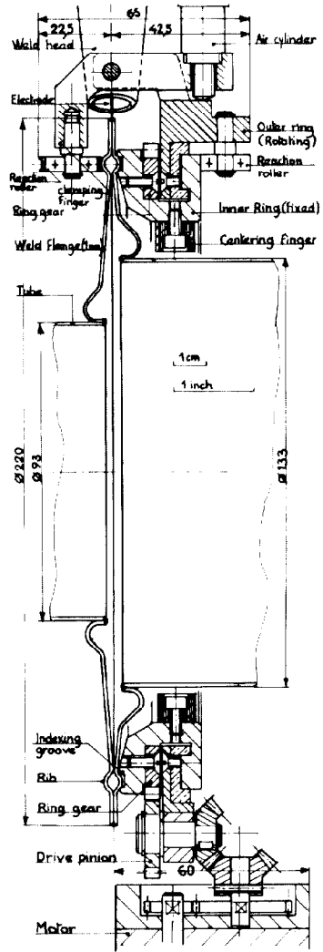
Fig. 2. Automatic weld flange welder assembly.
