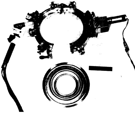
Fig. 4. Automatic welder in open position—ready for installation, and weld flange pair.
