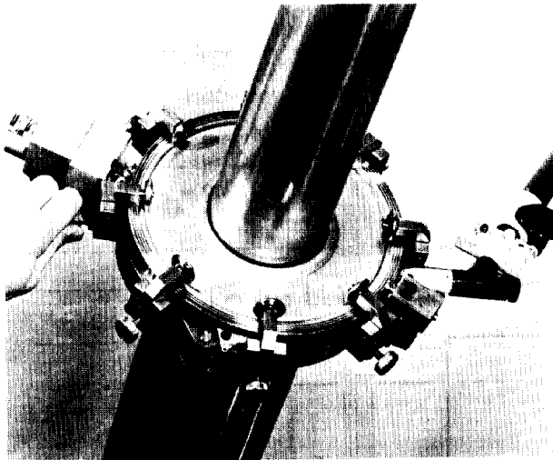
Fig. 3. Automatic welder shown in situ—on ISR beam transfer prototype vacuum system.
