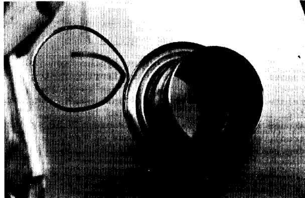
Fig. 9. Flange with machined groove for rip-off weld bead.
