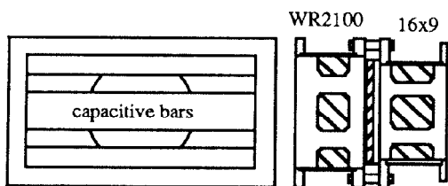
Figure 5. PEP II Traveling-wave window in WR2100 to 16x9 in waveguide transition
