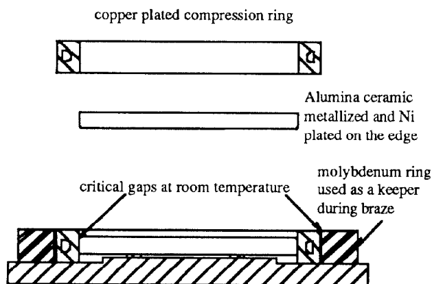
Figure 7. Window and compression ring assembly sequence
