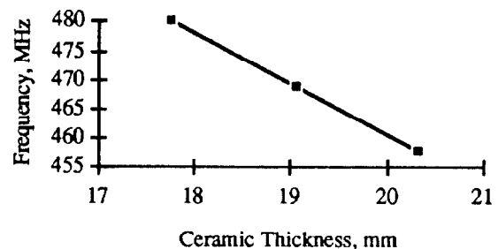
Figure 2. Match Frequency vs. Ceramic thickness for the 254 mm dia. self-matched window in 38 mm iris
