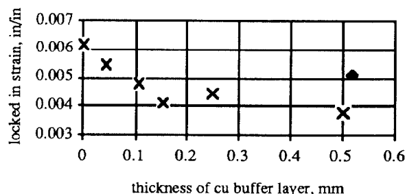
Figure 6. Braze test results for locked in strain after brazing for various thicknesses of buffer layer. Cool down from braze temperature was 1 °C per minute and, a) ♦ no hold period, b) x with a 10 hr hold period at 450 °C.
