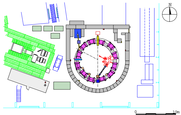
Figure 1: Layout of 150MeV FFAG synchrotron
