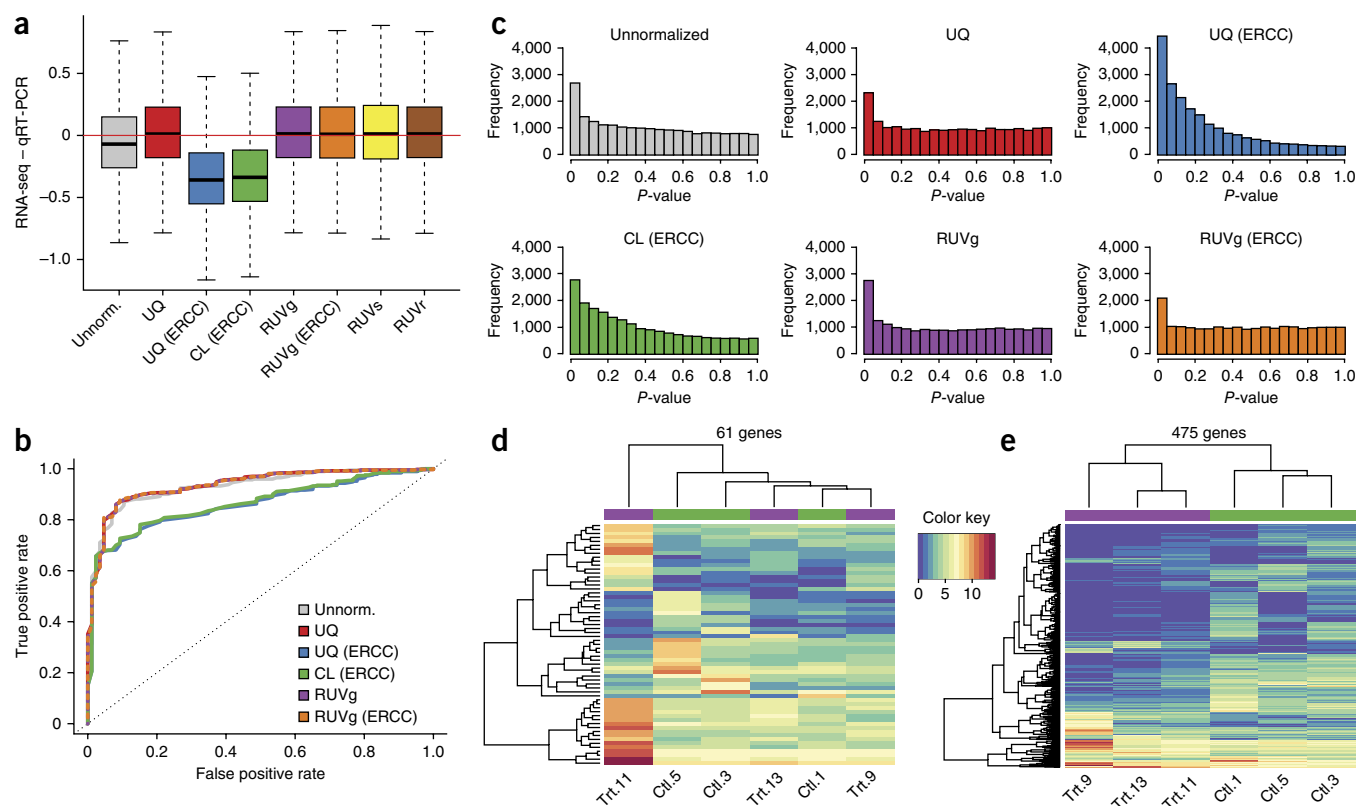
Figure 6 Impact of normalization on differential expression analysis. (a) For the SEQC data set, difference between RNA-seq and qRT-PCR estimates of sample A/sample B log-fold-changes, that is, bias in RNA-seq when viewing qRT-PCR as the gold standard. All RUV versions lead to unbiased log-fold-change estimates; cyclic loess (CL) normalization based on the ERCC spike-ins leads to severe bias. (b) For the SEQC data set, ROC curves using a set of 370 positive and 86 negative qRT-PCR controls as gold standard. RUVg (based on either empirical or spike-in controls) and UQ normalization perform slightly better than no normalization. UQ normalization based on spike-ins performs similarly to no normalization and CL normalization based on spike-ins performs the worst. (c) For the zebrafish data set, distribution of edgeR P -values for tests of differential expression between treated and control samples. UQ and CL normalization based on spike-ins lead to distributions far from the expected uniform. (d) For the zebrafish data set, heatmap of expression measures for the 61 genes found differentially expressed between control (Ctl) and treated (Trt) samples after UQ but not after RUVg normalization. Clustering of samples is driven by outlying library 11. (e) Heatmap of expression measures for the 475 genes found differentially expressed after RUVg but not after UQ normalization. Samples cluster as expected by treatment.
