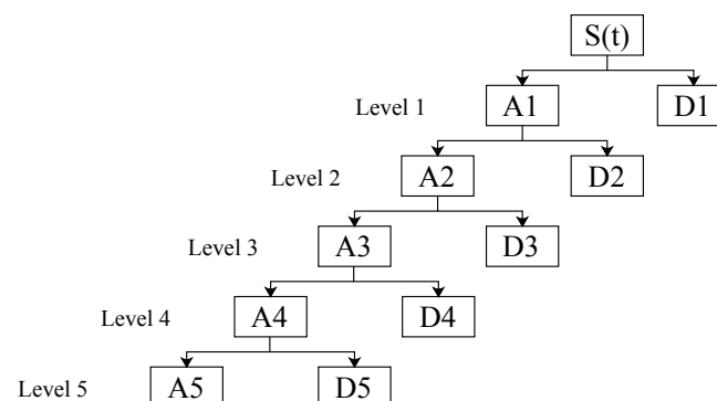
Figure 2. Decomposition wavelet in five levels: tree topology.
