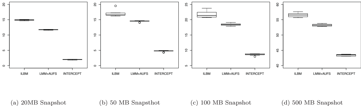
Figure 3: The average turnaround time in the cases of Incremental Live Block Migration(ILBM), Live Memory Migration with AUFS (LMM+AUFS), and Kemari-based Live Memory Migration with AUFS (INTERCEPT).
