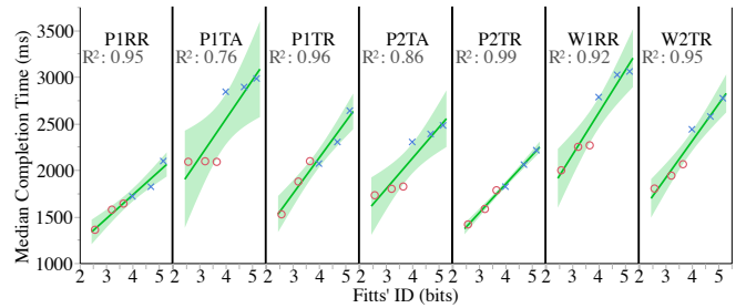
Figure 6. Median CT as a function of Fitts' ID per Technique, with corresponding confidence regions and R^2 . Circles and crosses are respectively 60 mm and 20 mm targets.
