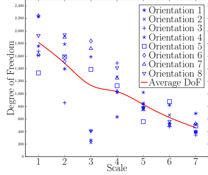
(b) Degrees of freedom for all orientations and scales.
