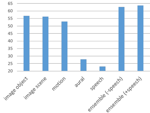
Figure 8: Accuracy of topic prediction with different modalities and ensembles. (-speech) and (+speech) means ensemble without and with speech modality.
