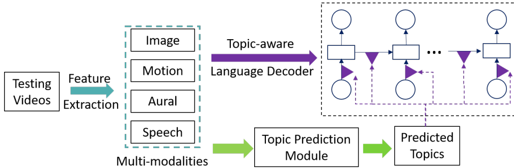
Figure 2: Framework of the proposed topic-guided model (TGM). We use the automatically mined topics as our topic guidance. For testing videos, multimodal features are utilized to predict the mined topics. Then the predicted topics are adopted in the topic-aware language decoder to generate topic-oriented video captions.
