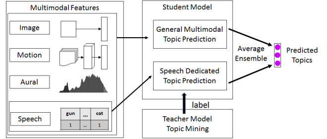
Figure 5: The framework for topic prediction. We treat the problem from a teacher-student perspective. The teacher topic mining model is used to guide the two student topic prediction models to learn based on general multimodalities and speech modality respectively.
