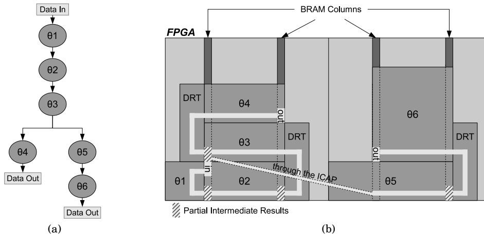
Fig. 1: Snake: a) Application task graph and b) Task allocation scheme
