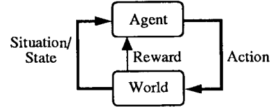
Figure 1: The Problem Formulation Used in Dyna. The agent's object is to maximize the total reward it receives over time. 1
