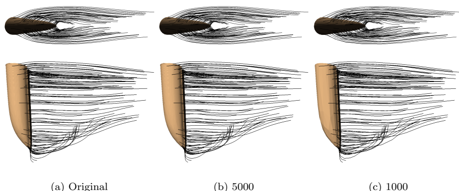
Fig. 27. Approximation of a simplicial complex containing 25,438 vertices. The model is an isosurface of the Liquid Oxygen Post data, with attached streamlines, and is pictured from both above and to the side.
