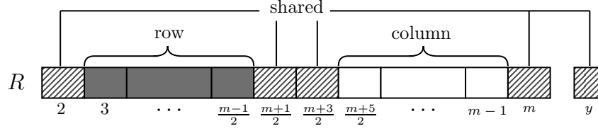
Figure 1: The partition of the randomness of Algorithm 5.5.
