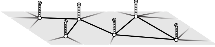
FIG. 5. Weighted reluctance to changing opinions may be modeled by extending the discourse sheaf over an augmented graph, giving each vertex a stubborn parent who exerts influence.
