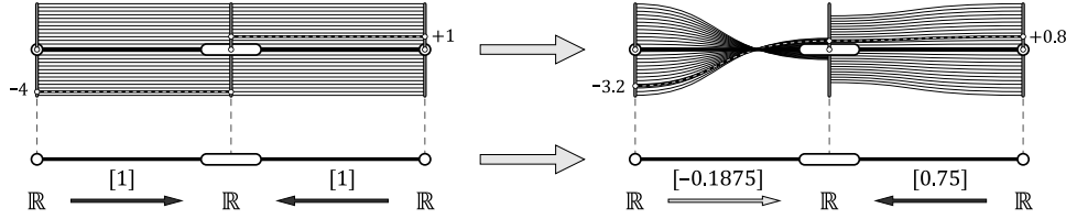
FIG. 7. A constant sheaf over an edge with an initial opinion distribution that is highly discordant [left] converges under the combined opinion-expression diffusion to a nonconstant sheaf [right] in which both opinions and expressions have relaxed to come to consensus. Under this initial condition, the agent on the left has learned to lie.
