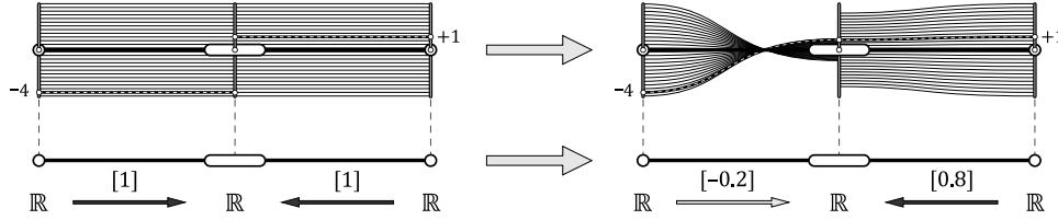
FIG. 6. A constant sheaf over an edge with an initial opinion distribution that is highly discordant [left] converges under diffusion of the sheaf to a nonconstant sheaf [right] in which the agent with the more extreme negative opinion has “learned to lie” in order to come to consensus.
