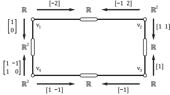
FIG. 2. A cellular sheaf over a simple cyclic graph. All stalks are of dimension one or two.
