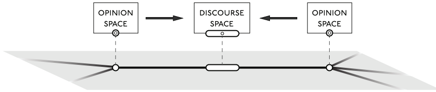
FIG. 3. In a discourse sheaf, stalks over vertices are individual opinion spaces, stalks over edges are discourse spaces, and restriction maps are expressions of opinions on the topics of discourse, formulated linearly from basis opinions.
