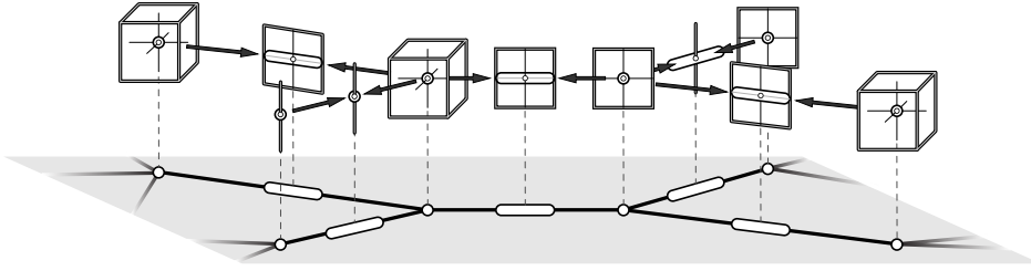
FIG. 1. A cartoon diagram of a cellular sheaf over a graph. Vector spaces of varying dimensions over vertices and edges are attached via linear transformations, following the adjacency pattern of the graph. The entire system of linear transformations forms the cellular sheaf.
