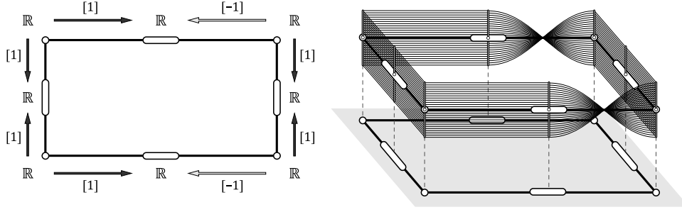
FIG. 4. A sheaf supporting stable polarized opinion distributions as global sections. The two agents on the right lie to their neighbors on the left, but are truthful to each other.
