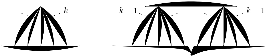
FIGURE 1. Two simple k -touching families of Jordan regions with chromatic number k + 1 .
