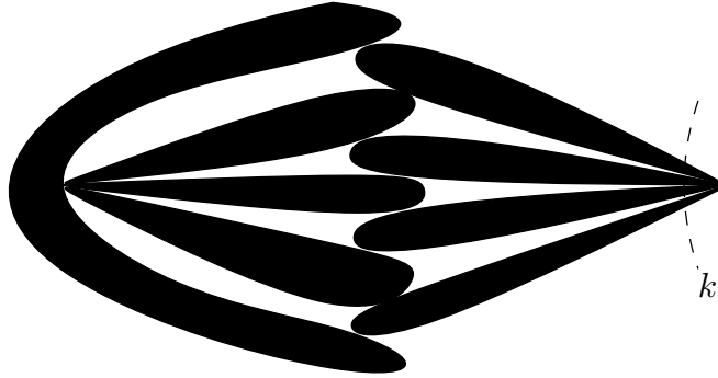
FIGURE 7. Every Jordan region intersects precisely k + 1 other Jordan regions.
