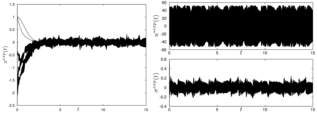
Figure 4: Time evolution of the control input u = u^{\text{nom}} - K\sigma - \gamma\sigma/(\|\sigma\| + 0.001) and the corresponding system trajectories and sliding variable with a sampling step h = 5 \text{ ms} .
