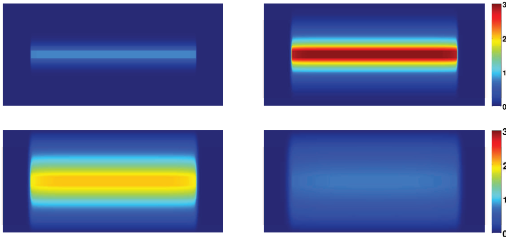
Figure 6.10: Snapshots of the multi-domain solution after 20,000 years (top left), 100 000 years (top right), 200 000 years (bottom left), and 1,000,000 years (bottom right), with a blow up in the y -direction.
