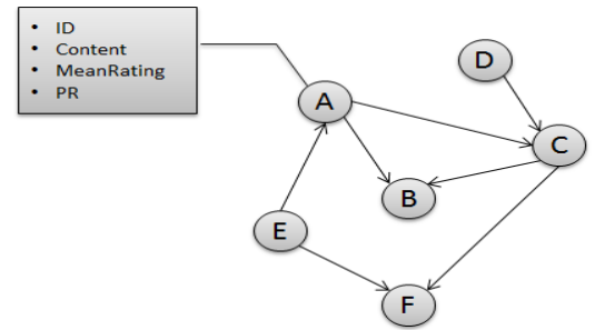
Fig. 3: Example of Directed Graph of Documents
