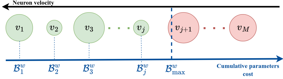
Figure 2. Selection of neurons to update given a network of M neurons and a budget \mathcal{B}_{\max}^w . The cost C_i^w is proportional to the size of the circle which represents the i -th neuron. The neurons selected for the update are in green, while those frozen in red.
