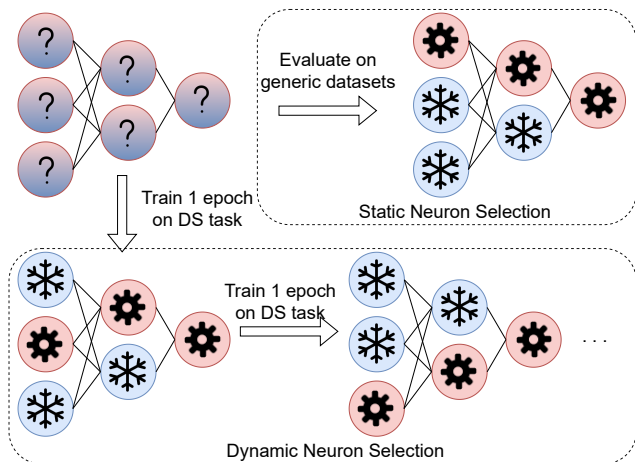
Figure 1. Comparison between static neuron update selection (up-right corner) and dynamic selection (down). While the static strategy evaluates the neurons to update on generic datasets and the sub-network will remain static for the whole training on the downstream (DS) task, with the dynamic selection it can change after every epoch.
