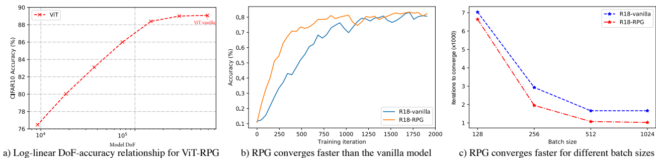
Figure 5: a) A log-linear DoF-accuracy relationship exists for RPGs applied to vision transformer ViT [17]. b) RPG converges faster than the vanilla model. We plot the CIFAR10 accuracy (smoothed by moving average) versus training iterations for Res18-vanilla and Res18-RPG. RPG converges at 1k iterations while the vanilla model converges at 1.7k. c) RPG consistently converges faster. The reduction becomes substantial with the increasing batchsize, e.g., at batchsize 1024, RPG takes 41% less iterations to converge. Denote final accuracy as P_f , the convergence iteration is defined when current smoothed accuracy (by moving average) is within 5% range of P_f .
