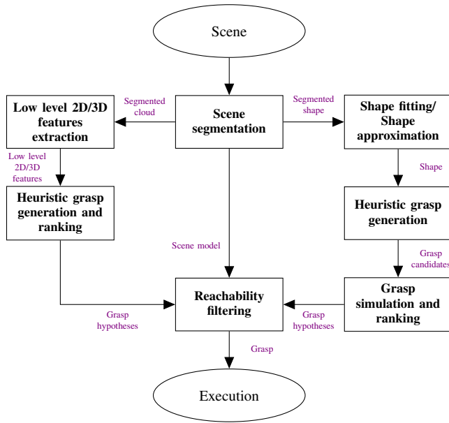
Figure 21: Typical functional flow-chart of a grasping system for unknown objects. The scene is perceived and segmented to obtain object hypotheses and relevant perceptual features. Then the system follows either the right or left pathway. On the left, low level features are used to generate heuristically a set of grasp hypotheses. On the right, a mesh model approximating the global object shape is generated from the perceived features. Grasp candidates are then sampled and executed in a simulator. Classical analytic grasp metric are used to rank the grasp candidates. Finally non reachable grasp hypotheses are filtered out, and the best ranked grasp hypothesis is executed. The following approaches use the left pathway: [116, 117, 119, 37, 33, 60, 121, 34, 122, 126]. The following approaches estimate a full object model: [118, 120, 110, 123, 124, 125]
