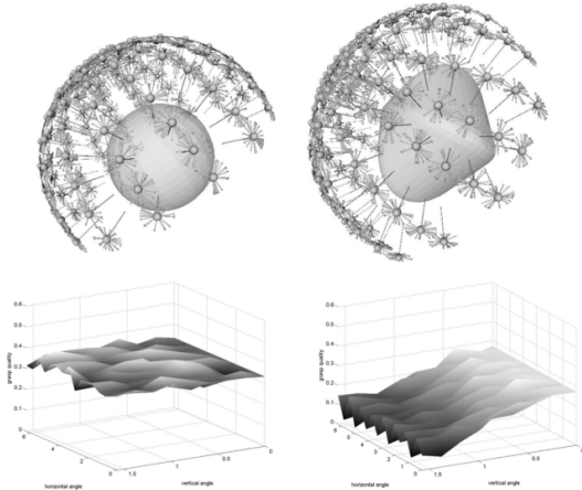
Figure 11: Top) Grasp candidates performed on SQ. Bottom) Grasp quality for each candidate [20].
