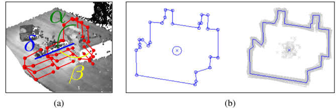
Figure 26: Mapping global object shape to grasps. 26a) Simplified hand model and grasp parameters to be optimized [122]. 26b) Planar object shape uncertainty model (Left) Vertices and center of mass with Gaussian position uncertainty ( \sigma = 1 ). Right) 100 samples of perturbed object models [125].
