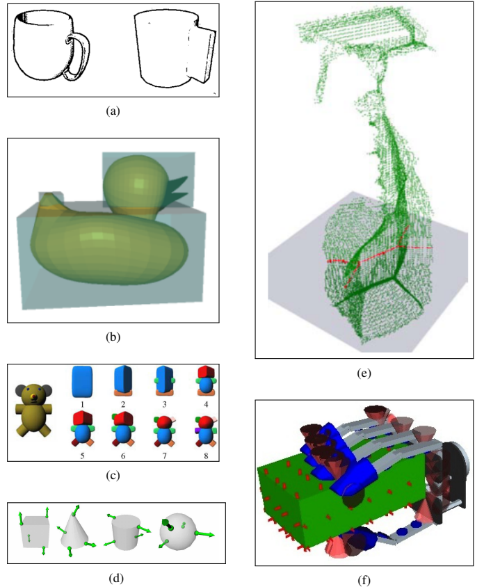
Figure 4: Generation of grasp candidates through object shape approximation with primitives or through sampling. 4a) Primitive Shape Decomposition [19]. 4b) Box Decomposition [67]. 4c) SQ Decomposition [21]. 4d) Randomly sampled grasp hypotheses.[22]. 4e) Green: Centers of a union of spheres. Red: Centers at a slice through the model [68, 56]. 4f) Grasp candidate sampled based on surface normals and bounding box [69].
