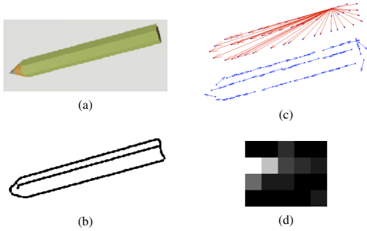
Figure 14: Example shape contexts descriptor for the image of a pencil. 14a) Input image. 14b) Canny edges. 14c) Top) All vectors from one point to all other sample points. Bottom) Sampled points of the contour with gradients. 14d) Histogram with four angle and five log-radius bins comprising the vectors in 14c Bottom) [32].
