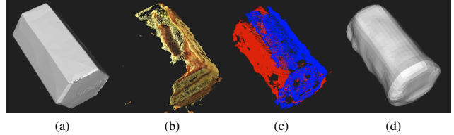
Figure 22: Estimated full object shape by assuming symmetry. 22a) Ground Truth Mesh. 22b) Original Point Cloud. 22c) Mirrored Cloud with Original Points in Blue and Additional Points in Red. 22d) Reconstructed Mesh [120].
