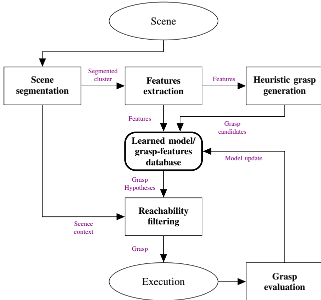
Figure 18: Typical functional flow-chart of a system that learns from trial and error. No prior knowledge about objects is assumed. The scene is segmented to obtain object clusters and relevant features are extracted. A heuristic module produces grasp candidates from these features. These candidates are ranked using a previously learned model or based on comparison to previous examples. The resulting grasp hypotheses are filtered and one of them is finally executed. The performance of the execution is evaluated and the model or memory is updated with this new experience. The following approaches can be summarized by this flow chart: [90, 71, 95, 104, 5, 26, 25]
