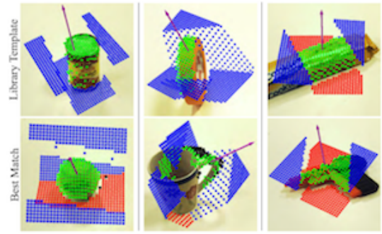
Figure 19: Example query and matching templates [71].
