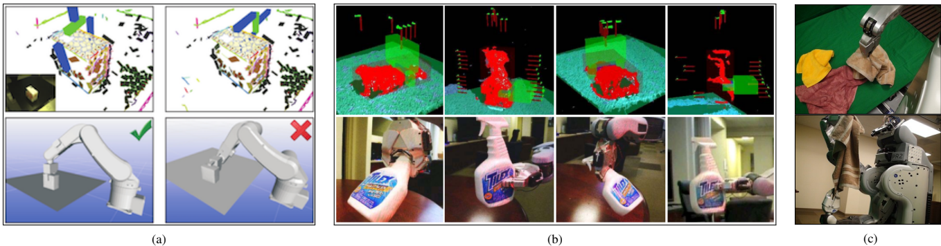
Figure 24: Generating and ranking grasp hypotheses from local object features. 24a) Generation of grasp candidates from local surface features and evaluation in simulation [117]. 24b) Generated grasp hypotheses on point cloud clusters and execution results [33]. 24c) Top) Grasping a towel from the table. Bottom) Re-grasping a towel for unfolding [37].
