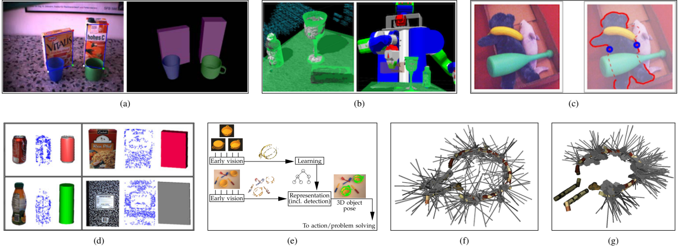
Figure 8: Object representations for grasping and corresponding methods for pose estimation. 8a) Object pose estimation of textured and untextured objects in monocular images [73]. 8b) ICP-based object pose estimation from segmented point clouds [75]. 8c) Deformable object detection and pose estimation in monocular images[55]. 8d) Multi-view object representation composed of 2D and 3D features [63]. 8e) Probabilistic and hierarchical approach towards object pose estimation [72]. 8f) Grasp Candidates linked to groups of local contour descriptors. [27]. 8g) Empirical grasp density built by trial and error. [27]
