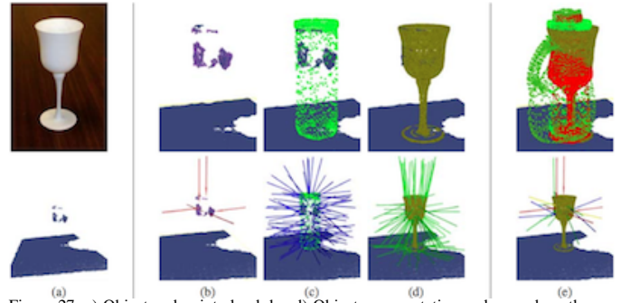
Figure 27: a) Object and point cloud. b,c,d) Object representation and grasp hypotheses. e) Overlaid representations and list of consistent grasp hypotheses [60, 127].
