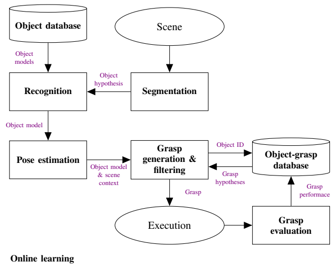
Figure 7: Typical functional flow-chart of a system that learns through trial and error. First, a known object in the scene is segmented and recognized. Past experiences with that object are retrieved and a new grasp hypothesis is generated or selected among the already tested ones. After execution of the selected grasp, the performance is evaluated and the memory of past experiences with the object is updated. The following approaches use trial-and-error learning: [27, 58, 64, 66].
