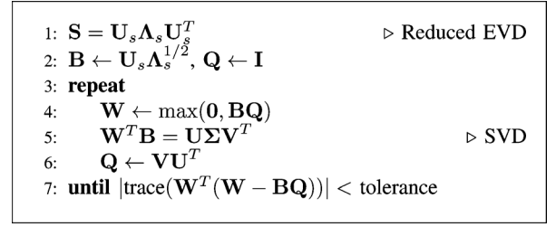
Fig. 4. Proposed algorithm for symmetric NMF.
