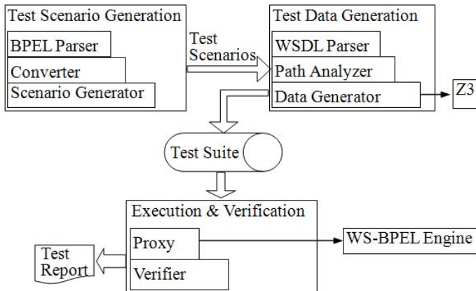
Fig. 5. The architecture of the prototype tool
