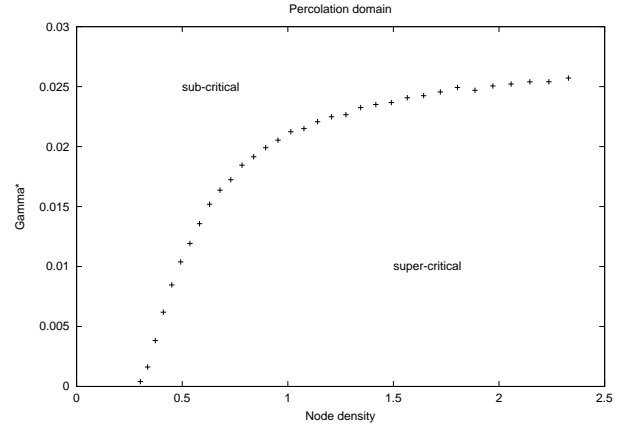
Fig. 10. Critical value of \gamma for an unbounded attenuation function L(\mathbf{x}) = ||\mathbf{x}||^{-3} . In this case, the percolation threshold is an increasing function of the node density. [The parameters of this simulation are \beta = 1 , N_0 = 10^4 and P_i = 10^5 \forall i .]
