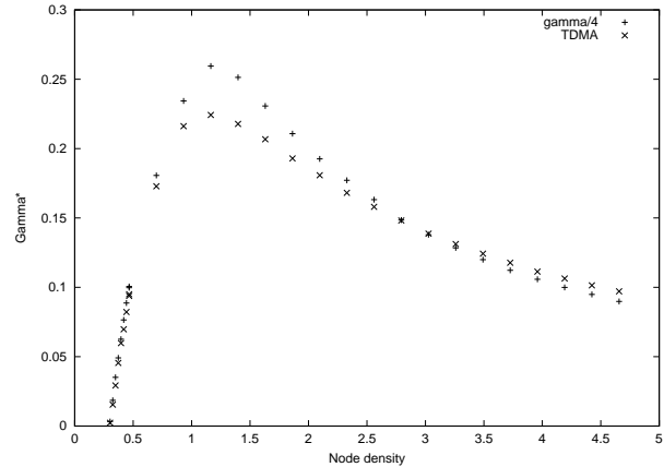
Fig. 11. Comparison between the critical threshold in the TDMA case ( n = 4 time slots) and in the original model with all nodes allowed to emit simultaneously. To make comparison easier, the critical value in the second case has been multiplied by 4. [Simulation parameters are the same as in Figure 3]
