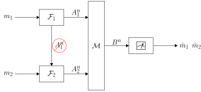
Fig. 1. The quantum multiple-access channel \mathcal{M}_{A_1 A_2 \rightarrow B} with cribbing at Encoder 2.
