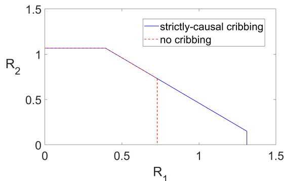
Fig. 3. Achievable regions for the single-mode bosonic MAC. The decode forward achievable region with strictly-causal cribbing is the area below the thick blue line (see (42)). For comparison, the capacity region without cribbing \mathcal{C}_{\text{none}}(\mathcal{N} \circ \mathcal{L}) is depicted as the area below the red dashed line (see (44)). The transmission rate of Alice 1 can be significantly higher using cribbing.
