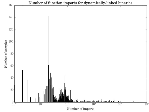
Fig. 5. Number of imported symbols in dynamically linked samples
