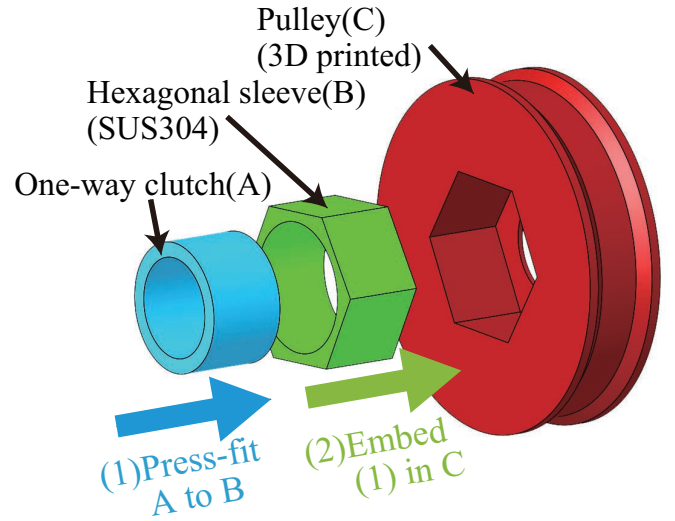
Fig. 10. Design concept of tensioner.
