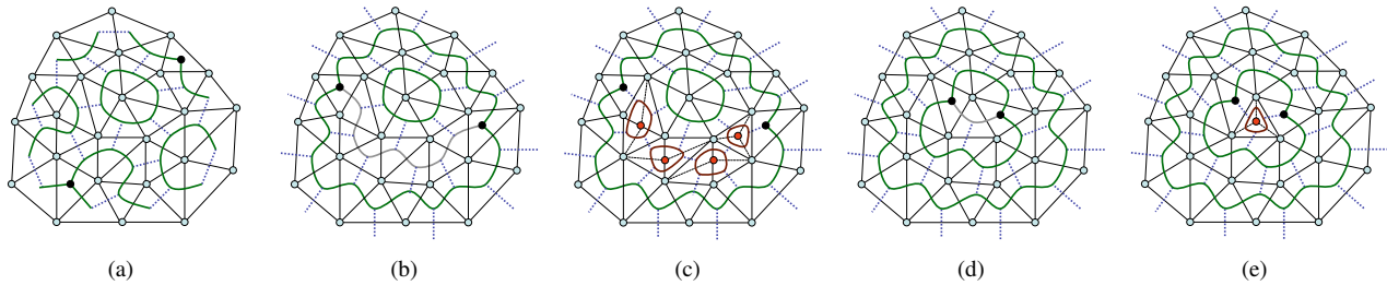
Figure 3. (a) The stripification algorithm of [4] produces linear strips and strip loops in a mesh with boundary. (b) Forcing matching of the boundary triangles produces unmatched triangles (also called junction nodes, denoted by dark points) and paths of unmatched edges between them. The shortest path is shown using a lighter color. (c) The internal triangles along this shortest path are paired. Each pair of triangles is split into four triangles. Triangles without a pairing are split into three triangles. This yields perfect matching of the entire mesh. The number of new triangles introduced is dependent on the length of the shortest path. (d) An alternate matching yielding a shorter path between the junction nodes. Such shortest paths are produced by (optimal) forced-loop algorithm. (e) The only triangle in the shortest path, and hence without a pair, is split into three triangles as before.
