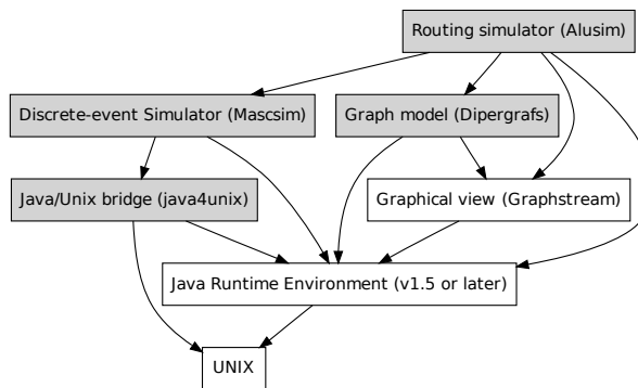
Figure 2: The dependencies of modules
