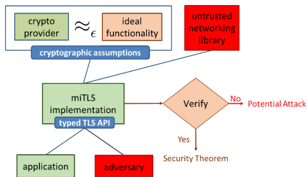
Figure 1: miTLS verification architecture
