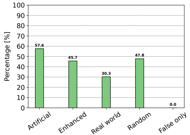
Fig. 9. False alarm rate of all models.
