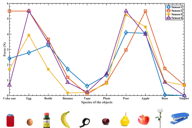
Fig. 10. The needed force for gripping different objects.
