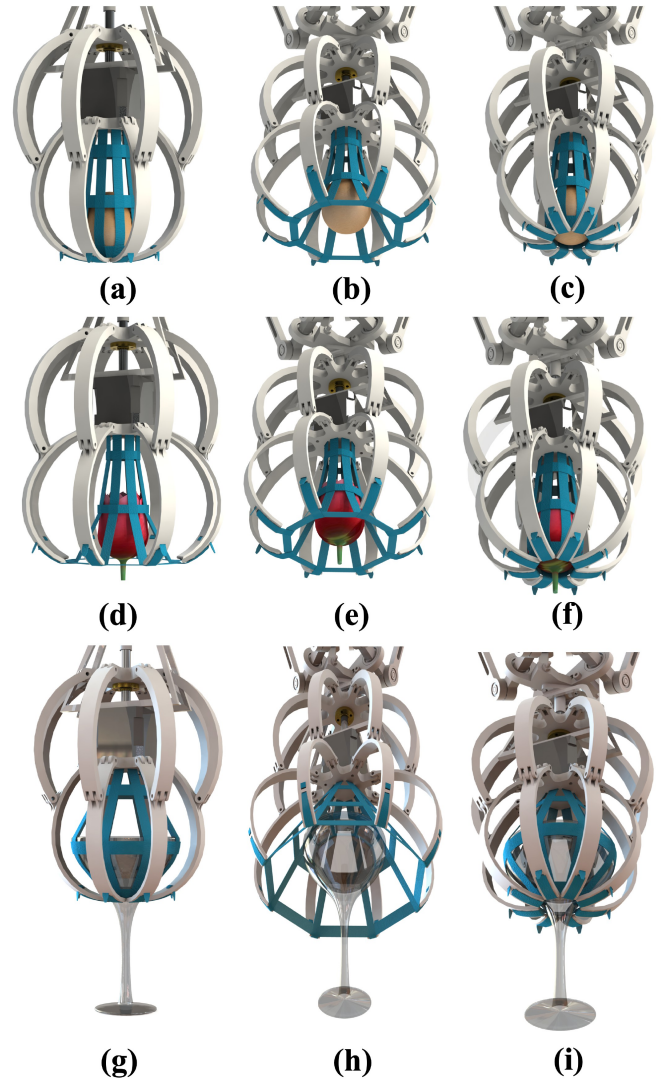
Fig. 6. Detailed processes of grasping egg, rose, and glass.
