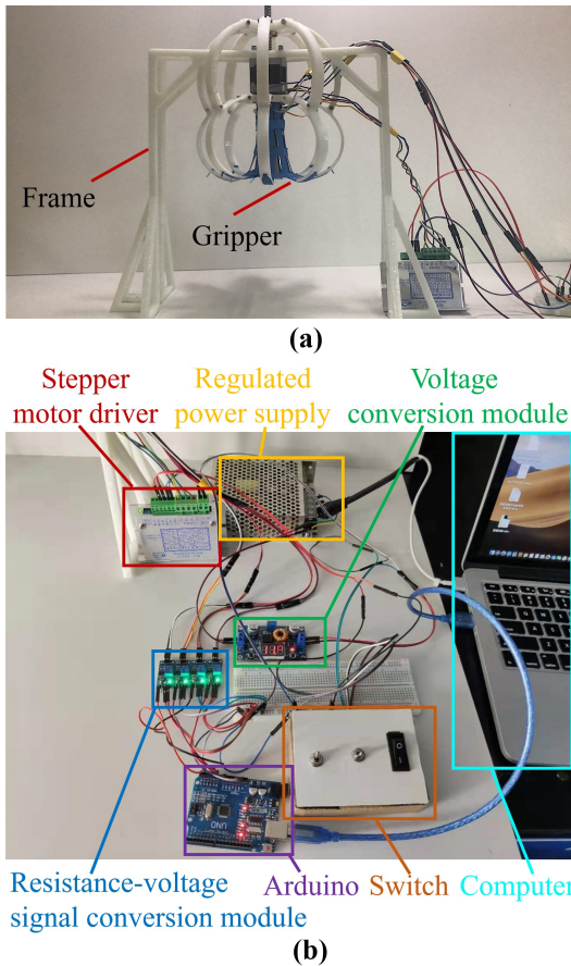
Fig. 4. Scene of test experiments of the gripper. (a) The gripper fixed on a frame. (b) Test circuit of the gripper.
