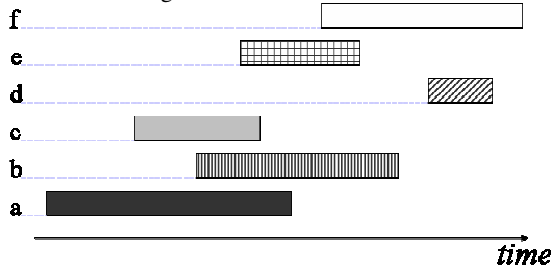
Figure 1: Data lifetime.
