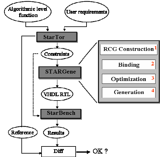
Figure 3: STAR design flow and associated tools.
