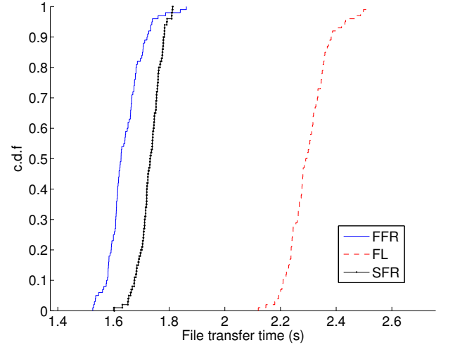
Fig. 6. Comparison of file transfer time achieved through multiple runs for FFR, FL and SFR, comparison between local and global optima
