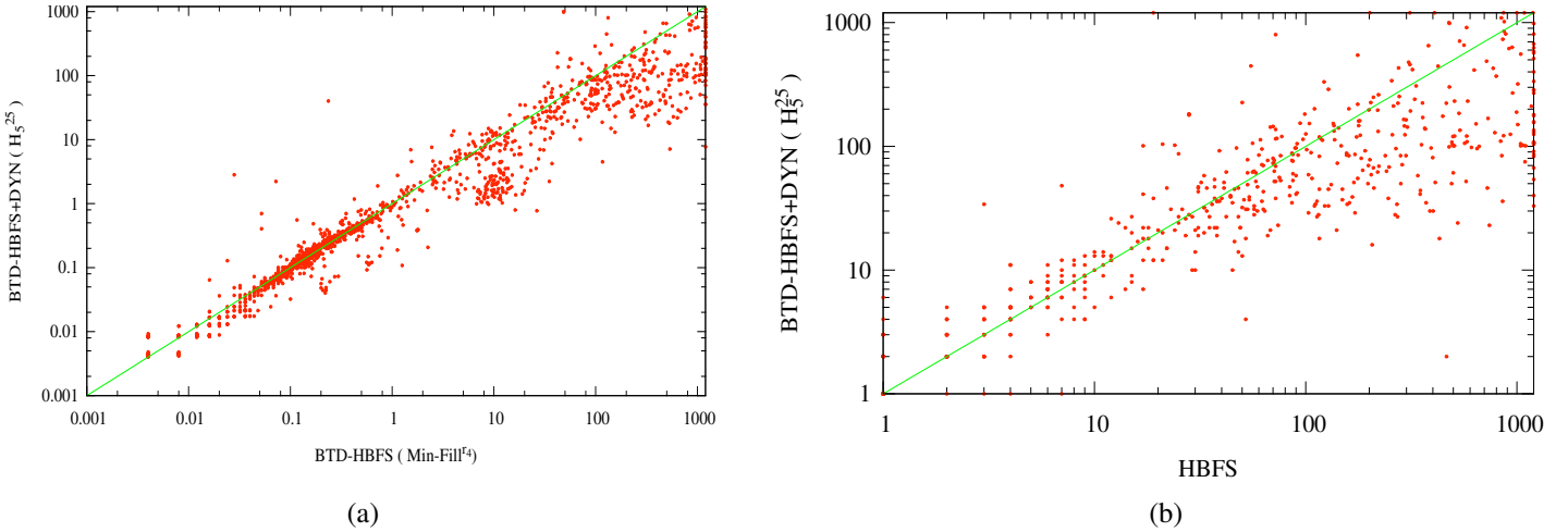
Fig. 5. (a) Runtime comparison between BTD-HBFS+DYN with H_5^{25} and BTD-HBFS with Min-Fill r4 (a) and HBFS (b).
