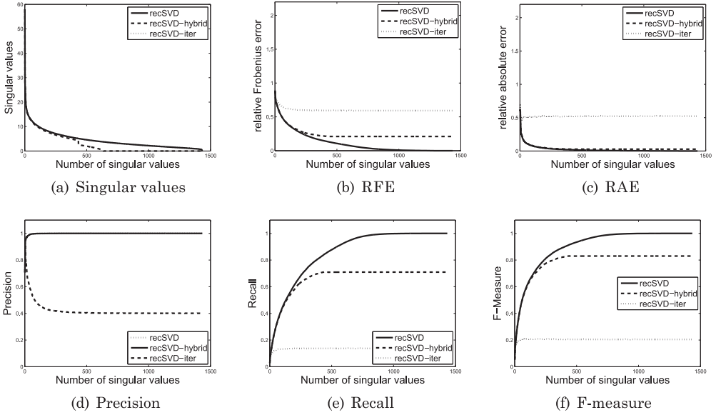
Fig. 5. CORA dataset. Performance of the RecSVD, Iterative, and Hybrid algorithms as a function of the number of singular values; x -axis: number of singular values; y -axis: magnitude of the singular values (a), RFE (b), RAE (c), precision (d), recall (e), and F-measure (f).
