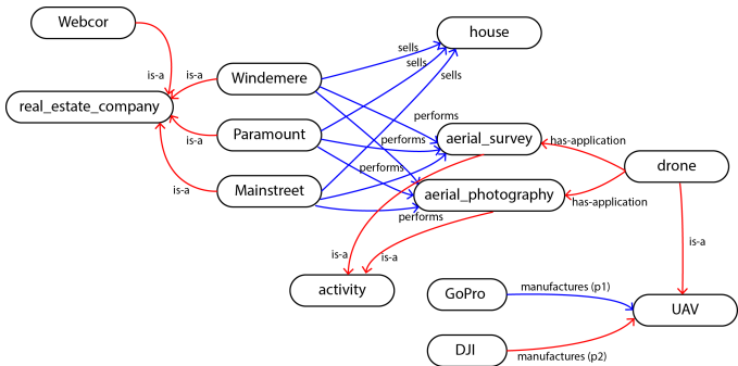
Figure 2: Example of a Knowledge Graph tracking emerging technologies.
