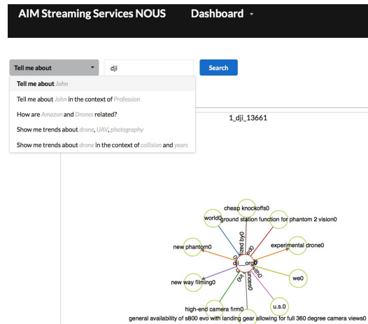
Figure 6: Web based interface for Trending, Entity and Relationship-based queries. The image here shows results for an entity query “Tell me about DJI”, where DJI is world’s leading company for manufacturing drones.
