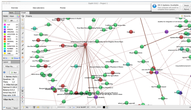
Figure 4: Visualization of a subgraph from a drone-themed Knowledge Graph. Algorithms in NOUS can be used to develop custom knowledge graphs for any arbitrary application domain.
