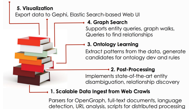
Figure 1: Various components of NOUS.
