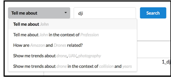
Figure 5: Five classes of natural language like queries that are transparently translated to execute distributed algorithms for subgraph pattern mining, entity-based queries or complex graph queries.
