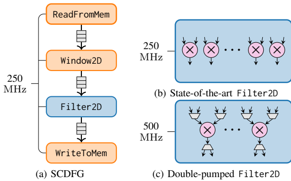
Fig. 1. Task-level multi-pumping saves resources at equal throughput for HLS of dataflow graphs (DFGs). The Filter2D task from a 2D Convolution kernel [10] (a) is double-pumped (c) by doubling its clock frequency and II to save half of the multipliers of the single-clock solution (b).
