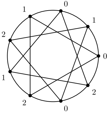
Fig. 6. The graph D_9 with a 3-colouring h_9 .
