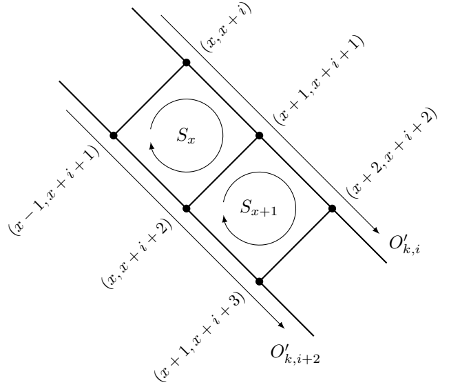
Fig. 5. Proof of Case 1 of Lemma V.8.
