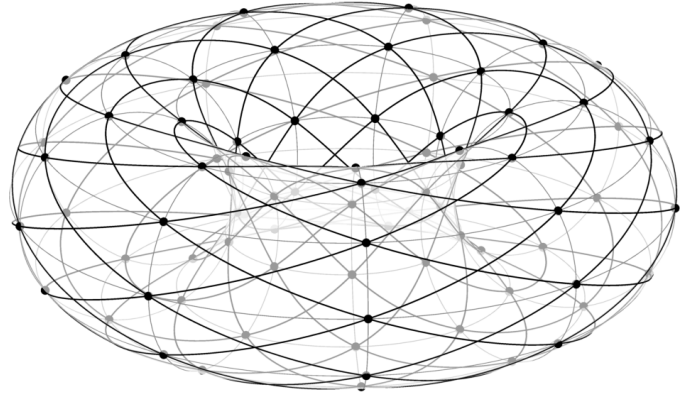
Fig. 3. The graph \mathbf{C}_9^2 on a torus.
